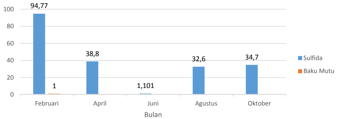
21.Sulfida (mg/L)
